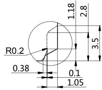
△1 Detail Q
